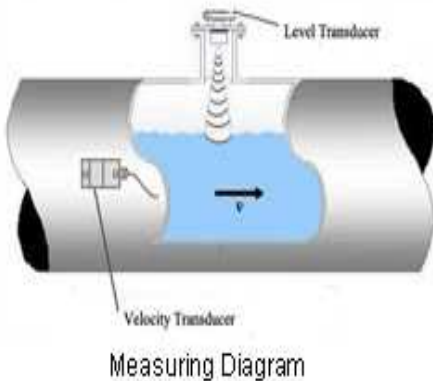
Velocity and Level Measurement (insertion)
